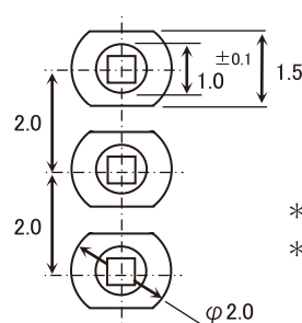
<3 lead pin type/2.0mm pitch>
