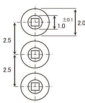
<3 lead pin type/2.5mm pitch>
